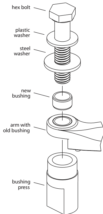
Fig. 3 - Use bushing replacement tools as shown to replace bushings on each arm.
