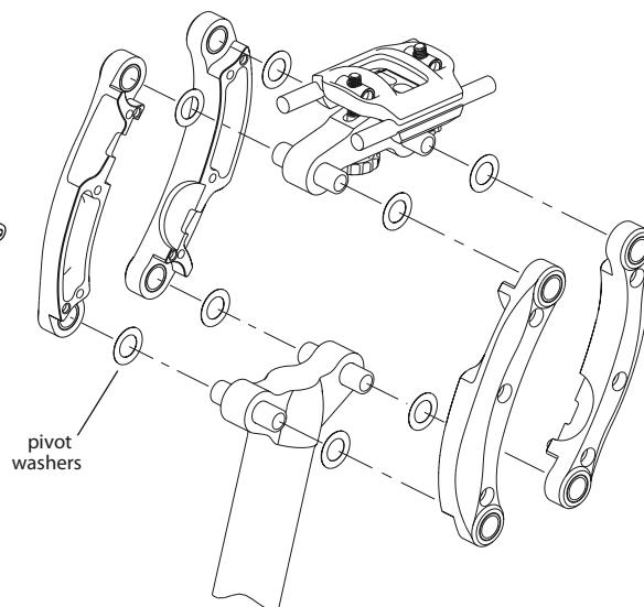
Fig. 3 - Remove arms and pivot shims from post (saddle clamp may need to be loosened)
